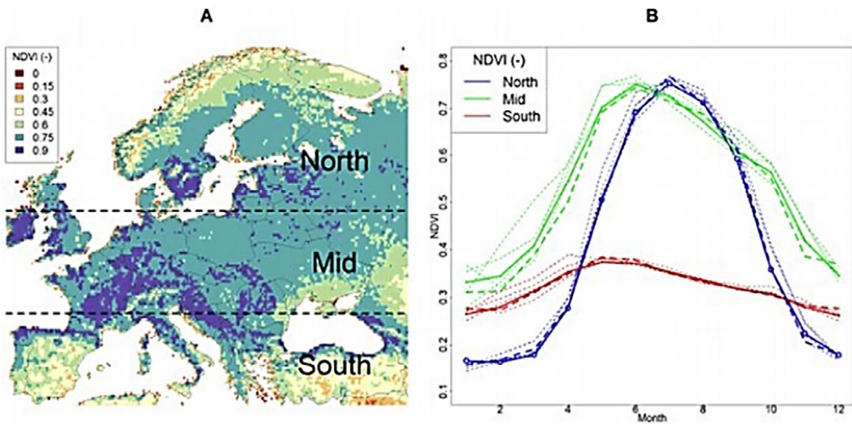
NDVI in Europe: (a) average values of NDVI for April to September in 1982–2010. (b) Continuous lines: average monthly values of NDVI in the latitudinal bands delineated in (a) ; the thin dashed lines are for the years 2001, 2002, 2004 and 2005, the bold dashed line is for 2003.
